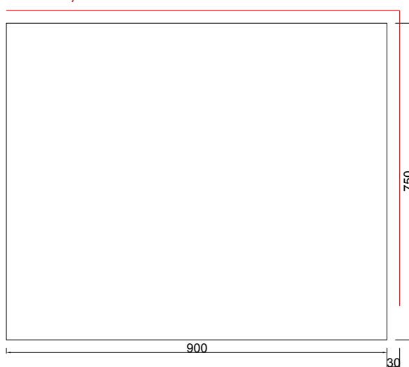
Chimney connection
